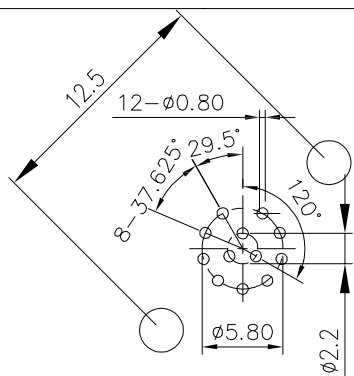
PCB layout
