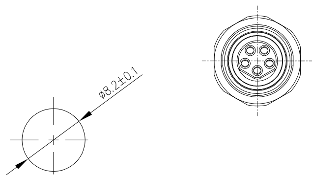
Panel cut
