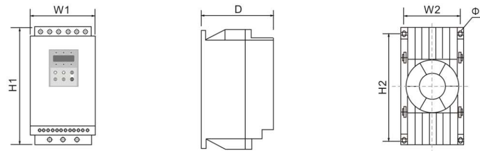
Soft Starter Outline & Mounting Dimension(Unit:mm)
