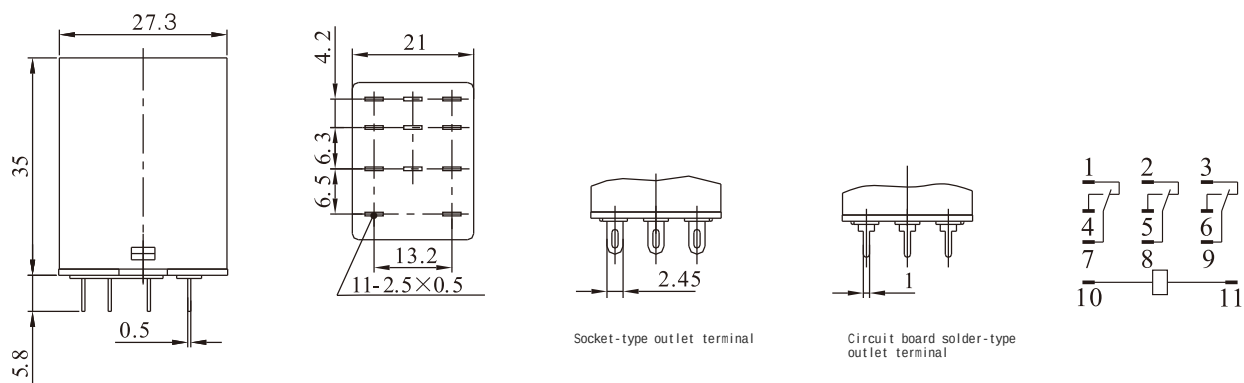
HHC68B-3Z(HH53P)
