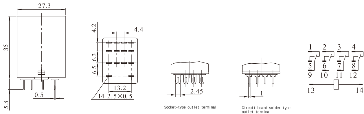
HHC68B-4Z(HH54P)
