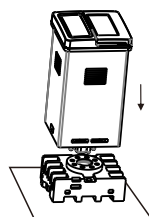
(15) Installation: install the relay, and align the upper boss with the groove on the base
