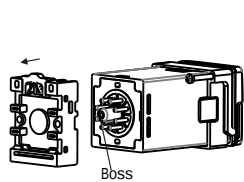
(1) Pull out the base and cover
