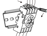
(13) Rail-type disassembly: remove the base
