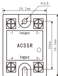
Installation Dimensions (Unit: mm)
