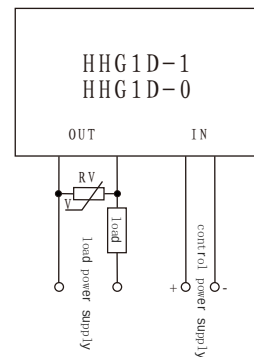
Wiring Diagram
