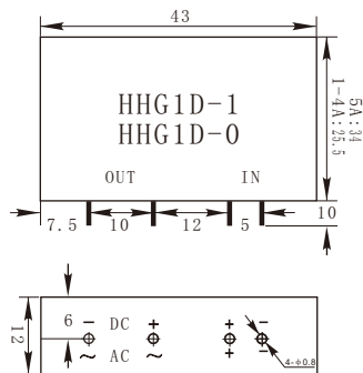
Installation Dimensions (Unit: mm)
