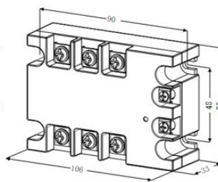
HHG1-3/032F-38 HHG1-3/250F-38
