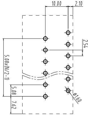
PCB LAYOUT
