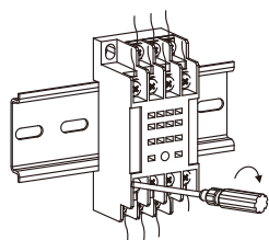
(8) Connect wires according to the base terminal numbering and tighten the terminal screws
