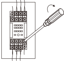
(2) Connect wires according to the base terminal numbering and tighten the terminal screws.
