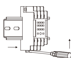
(12) Pry open the rail clip and remove the base.
