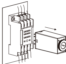
(4) Pull out the relay.
