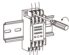
(11) Loosen the terminal screws and remove the wires.
