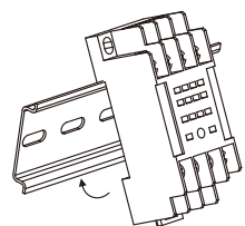
(7) Snap the base onto the rail.
