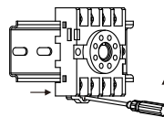
(12) Rail - type Disassembly: Pry open the Rail Clips and Remove the Base
