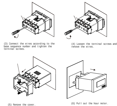
(5) Remove the cover.
