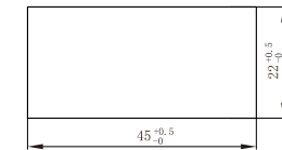
Panel cutout dimensions
