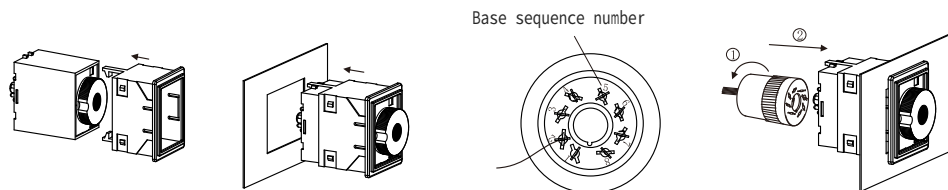
(9) Panel - type installation: Pass the wire through the back cover of the lamp holder base, solder the wire according to the base sequence number. The soldering time should not be too long, and each terminal needs to be put on an insulating bushing.
