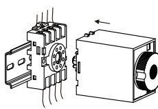
(6) Rail - type installation: Install the relay, and the protruding platform on the plug should align with the groove of the base.
