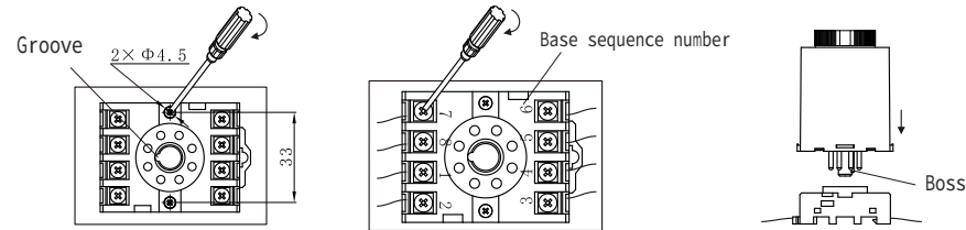
(1) Device - type installation: Tighten the installation screw.
