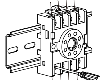
(5) Rail - type installation: Connect the wire and tighten the terminal screw.
