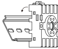
(4) Rail - type installation: Snap the base into the rail.
