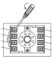
(5) Panel - mounting removal: Loosen the terminal screws and remove the wires.
