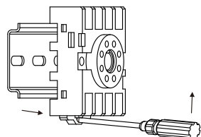
(12) Rail - mounting removal: Pry open the rail clip and remove the base.
