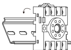
(7) Rail - mounting installation: Snap the base onto the rail.
