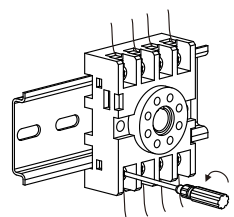
(11) Rail - mounting removal: Loosen the terminal screws and remove the wires.
