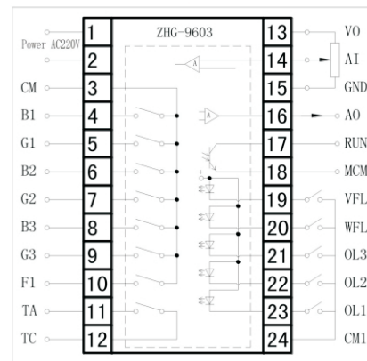
Picture 2-3 controller circuit terminal
