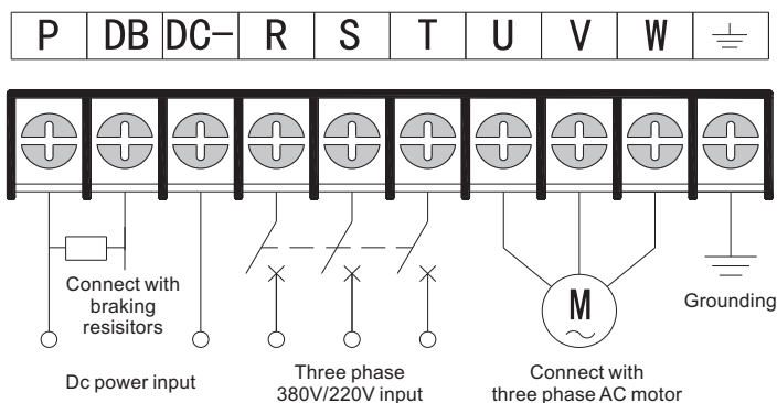
Fig. 3-4 Main Circuit Terminal 4
