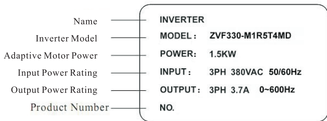
Fig.2-2 Inverter Label
