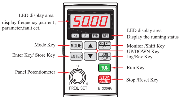
Fig.4-1 E-330MA operation panel
