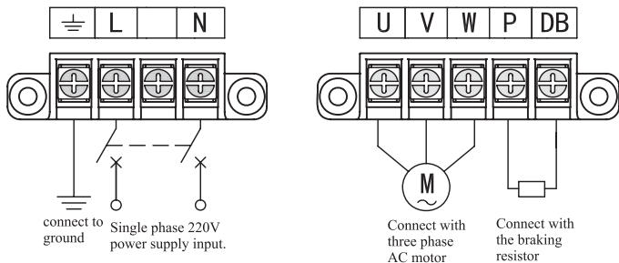
Fig.3-2 Diagram 1 for Main Circuit Terminal
