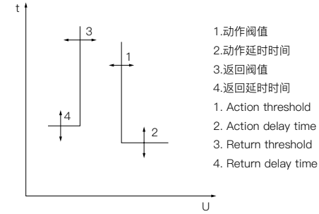
过电压保护动作原则 Overvoltage protection action principle
