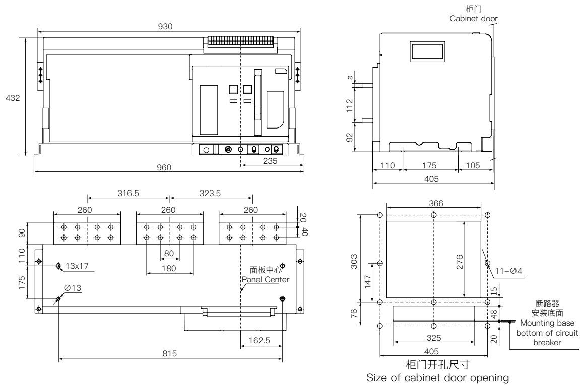
GYW6-6300(6300A) 抽屉式外形及安装尺寸 Shape and Mounting Dimensions of GYW6-6300 Drawout Circuit Breaker (6,300A)
