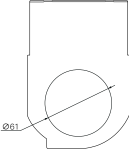
STW40壳架 Housing 2000~ 4000A
