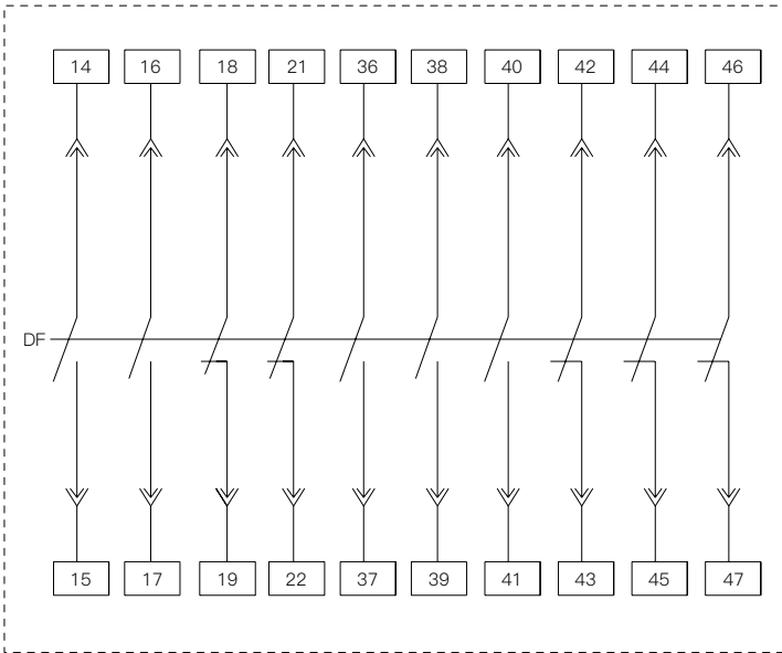
五常开五常闭（特殊配置） Five normally open and five normally closed (special configuration)
